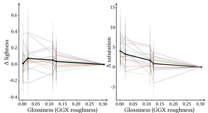
Figure 4: Average picked colors for every color-material pair, with error bars showing 1.0 standard deviation (faded), broken down into lightness and saturation using the CIECAM16 color appearance model. In black, average saturation and lightness across colors for every material, which showcases a strong correlation between perceived color saturation shift and gloss levels, while discarding any consistent lightness and gloss interaction.
