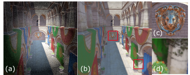
Figure 14: Gaze-contingent Adaptive Sampling by Stengel et al. [SGEM16]. Incorporating visual cues such as acuity, eye motion, adaptation and contrast, a perceptually-adaptive sampling pattern is computed and used for sparse shading (a). Fast image interpolation (b) achieves the same perceived quality at a fraction of the costs of shading each fragment. The resulting image contains high detail in the foveal region (c) and reduced detail in the periphery (d). Image from Stengel et al. [SGEM16]
