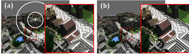
Figure 15: Ray Tracing-based foveated rendering in HMDs by Weier et al. [WRK*16] A gaze-adaptive and contrast-aware sampling is used to stochastically update pixels. The new samples are combined with reprojected samples from the previous frames to generate the final image (a). The presented user study shows, that even for small configurations of the foveal acuity, user's barely notice any difference to full rendering (b) Image from Weier et al. [WRK*16]
