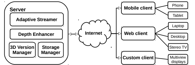
Figure 1: Design of the proposed 3D streaming system. The Depth Enhancer customizes the depth based on display sizes and viewing conditions. The creation of multiple versions of each 3D video is managed by the 3D Version Manager, and the storage of these versions is handled by the Storage Manager. The Adaptive Streamer uses DASH to serve segments of different versions to various clients.
