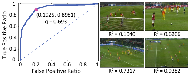
Figure 8: Left: ROC curve for our binary shot classifier. Right: Four examples of shots with corresponding R^2 values. Top two have low R^2 value, therefore, their depth will be unchanged. On the other hand, bottom two are long shots and due to the high R^2 value (above the threshold) their depth will be modified.
