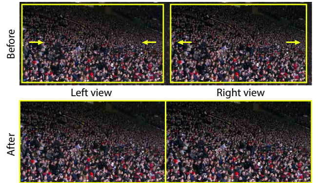
Figure 5: Example of the stretch operation. The left and right views are horizontally scaled. In effect, the horizontal component g_x of the disparity gradient g is changed.
