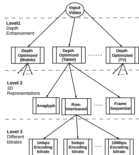
Figure 2: 3D Version Tree. It serves as an execution or master plan to create different versions of each 3D video.
