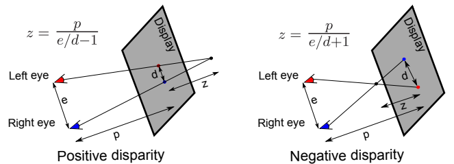
Figure 3: Disparity ( d ) vs. perceived depth ( z ). p is the viewing distance, and e is the inter-ocular distance.
