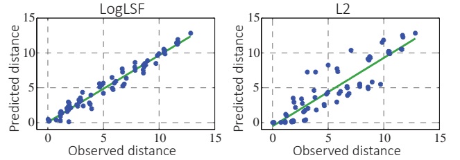
Figure 10: The two plots visualize the distance prediction between our stimuli as predicted by the LogLS model and the L2 norm with respect to the observed distances in the perceptual space. LogLSF outperforms the L2 norm by providing a much closer match to the observed distances.
